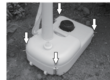
Base tank can be fixed on ground through four holes at the corner if necessary Pegs are sold separately, not included.
