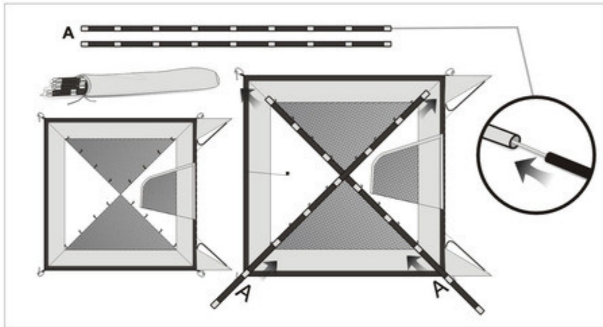
Fiberglass pole
