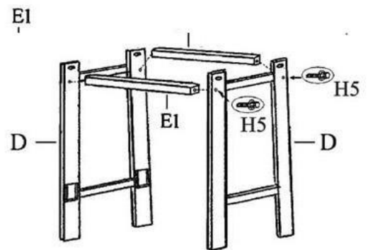
Step2 Keep all the screws loose at this time.
