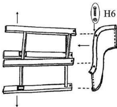
Step3 Keep all screws loose at this time.
