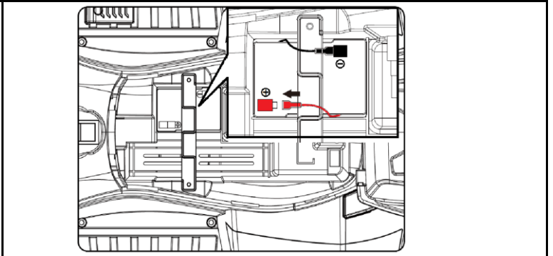
10.CONNECT THE BATTERY ELECTRIC LINE INTO THE BATTERY
