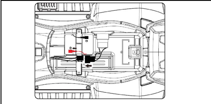
9.CONNECT THE MOTOR ELECTRIC LINE INTO THE MOTOR
