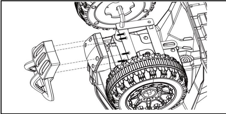
3.Install bumper(4X(4X10)SCREW)
