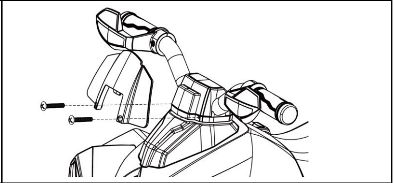
6.Fasten the windshield to the handlebar,(2X(4X10)SCREW)
