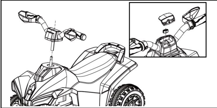
5.Insert handlerbar into the axial shaft ,secure with(1XM10 NUT)
